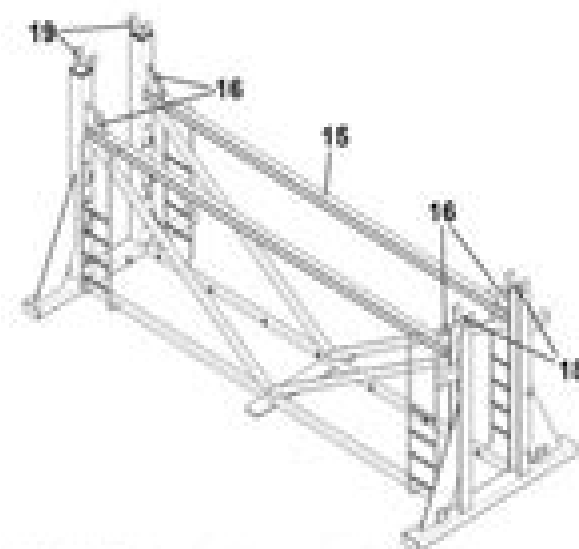
Fig. 3-115 Storing framework for the storage of a demolition attachment
