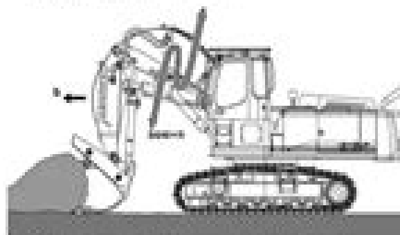
Fig. 3-77 Float position of the boom cylinders with a shovel attachment
