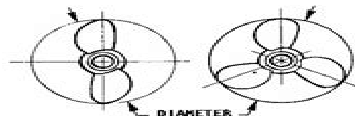
Diameter and pitch are the two basic dimensions of a propeller. The diameter is measured across the circumference of a circle scribed by the propeller blades, as shown.
