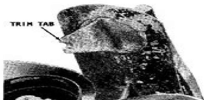
Zinc installation also used as the trim tab. The tab assists the helmsperson to maintain a true course without "fighting" the wheel.
