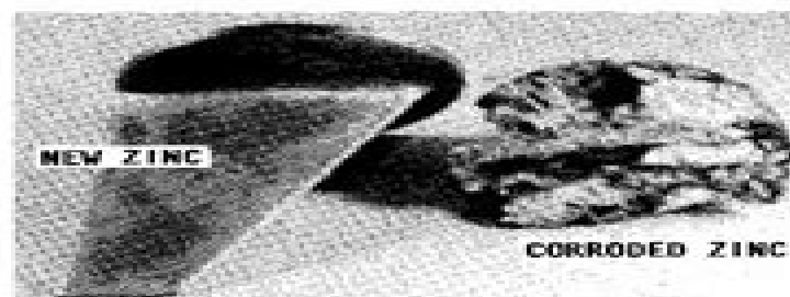
A new trim tab zinc, left, and a corroded zinc, right. An excellent example of the inexpensive zinc saving more costly parts of the outboard unit.
