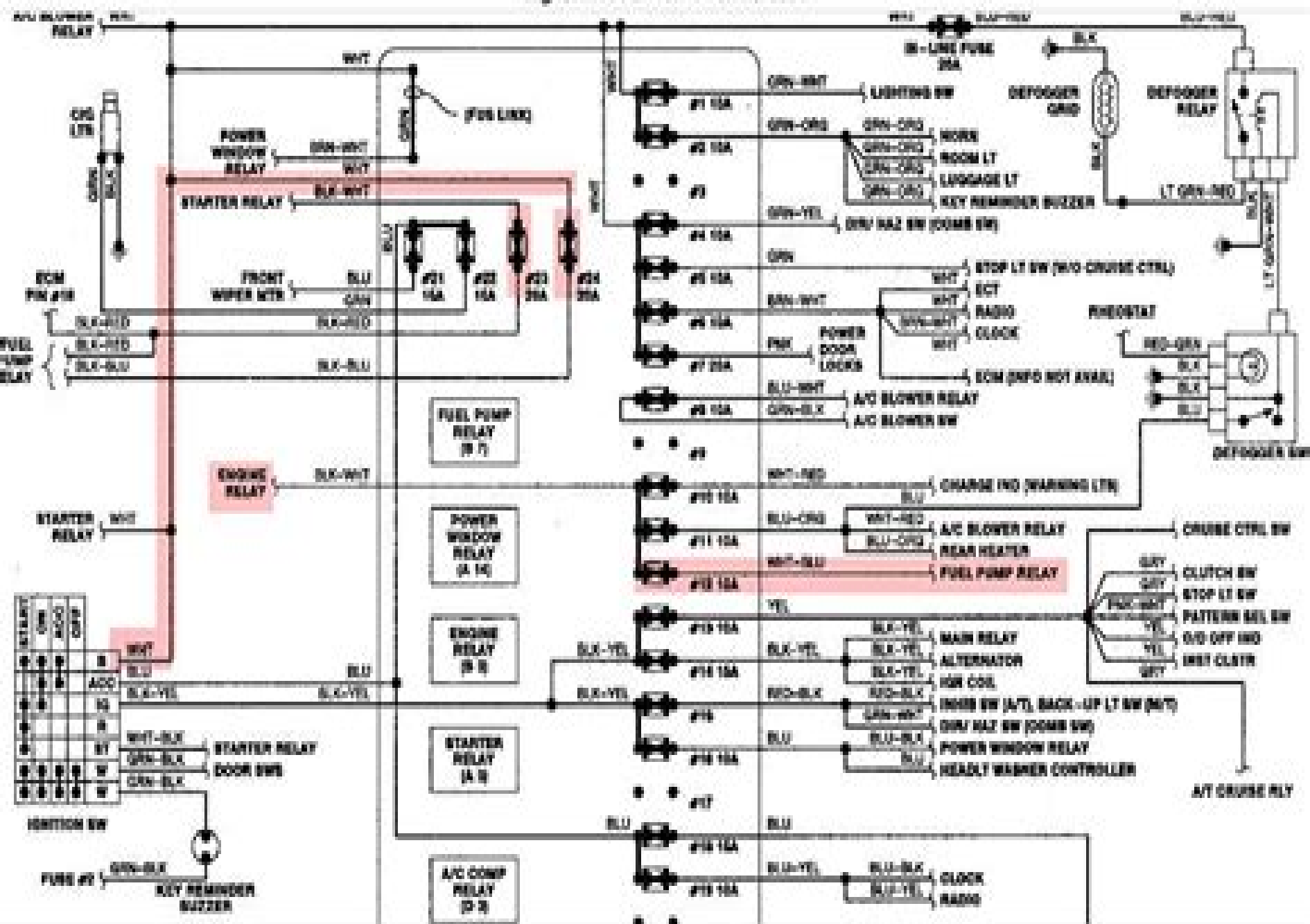
Fig. 3: Fuse Block & Underdash
