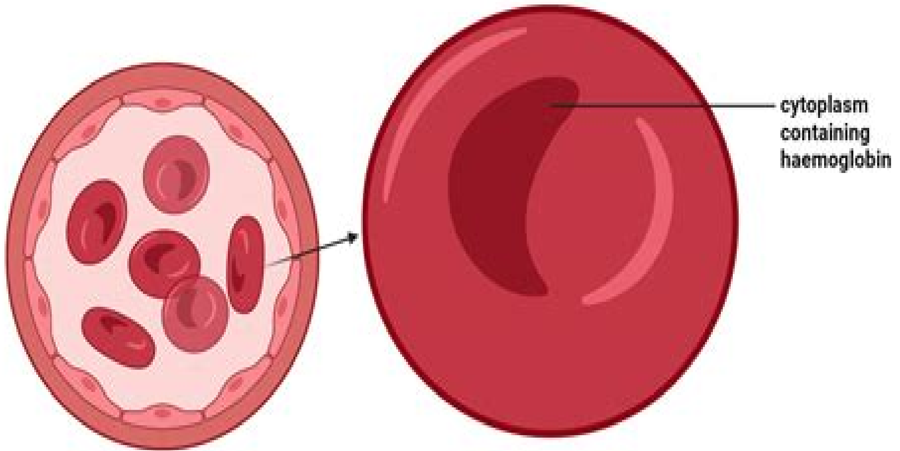
Vessel cross section with RBCs
