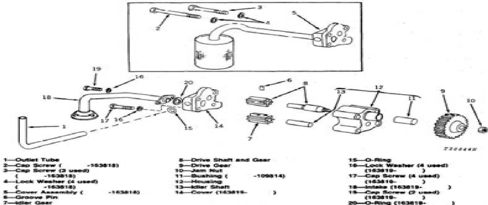
Fig. 3—Oil Pump
