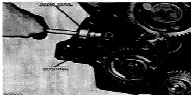
Fig. 4—Installing Pressure Regulating Valve Bushing
