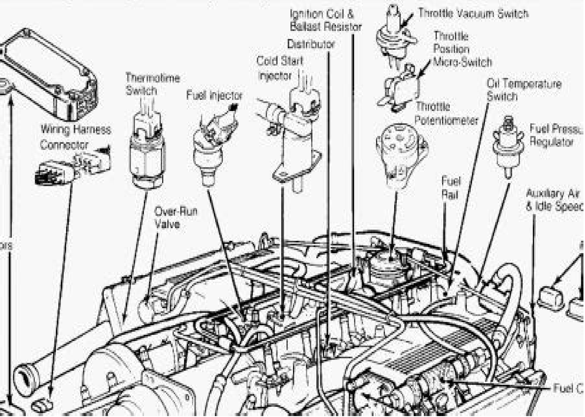
Fig. 1: Location of Engine Sensors and Components of EFI System Disconnect battery ground cable before disconnecting any components.
