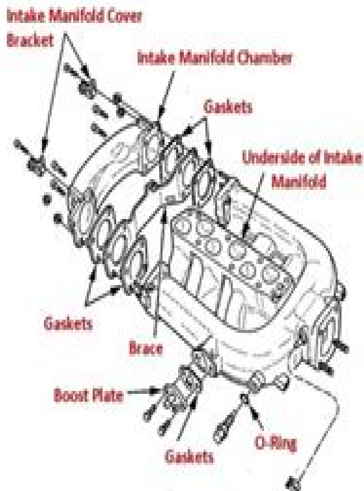
Intake Manifold
