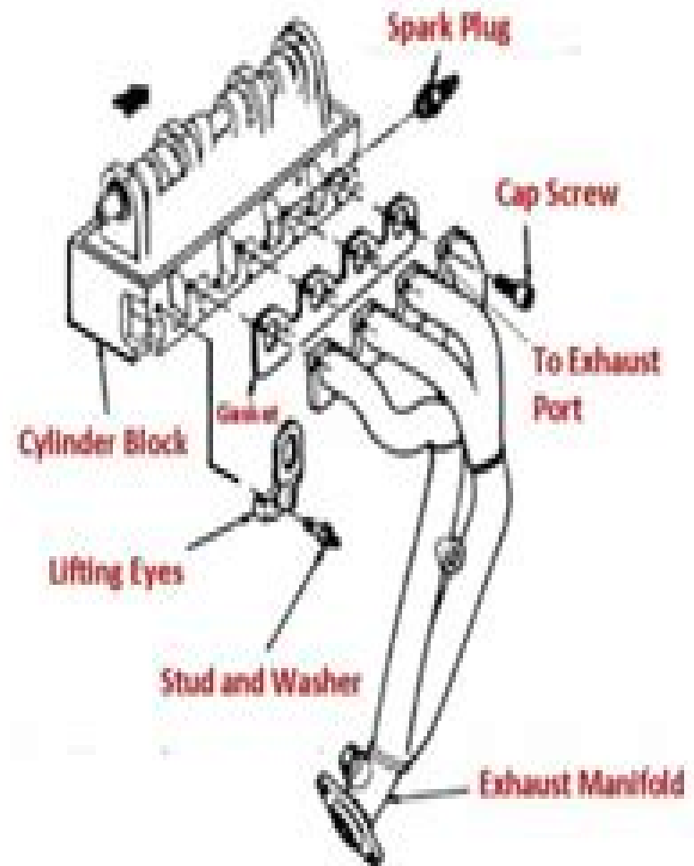
Exhaust Manifold
