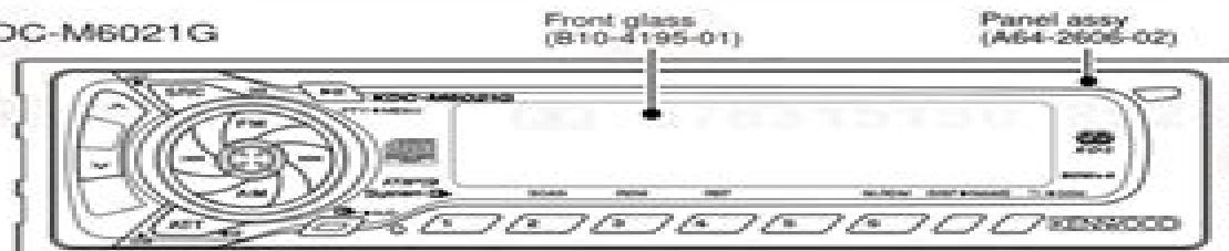
Mounting hardware assy (J21-9716-03)
