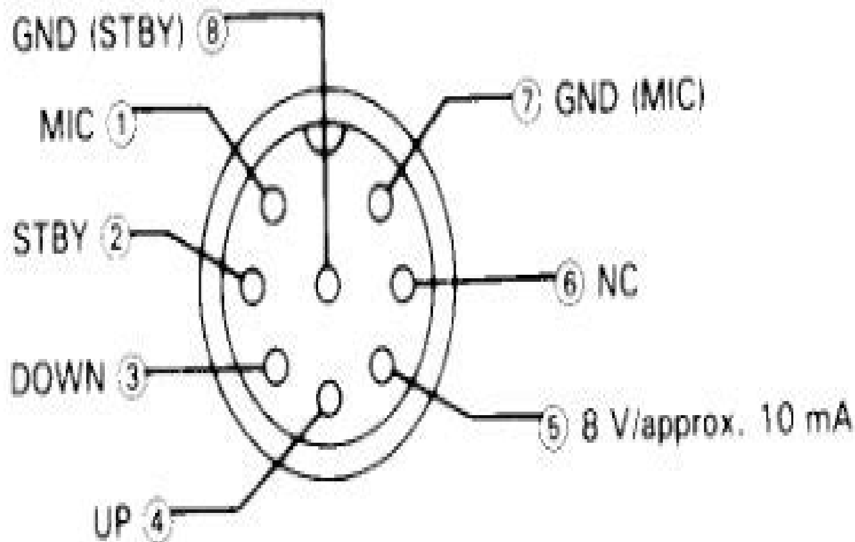
MIC connector (Front view)
