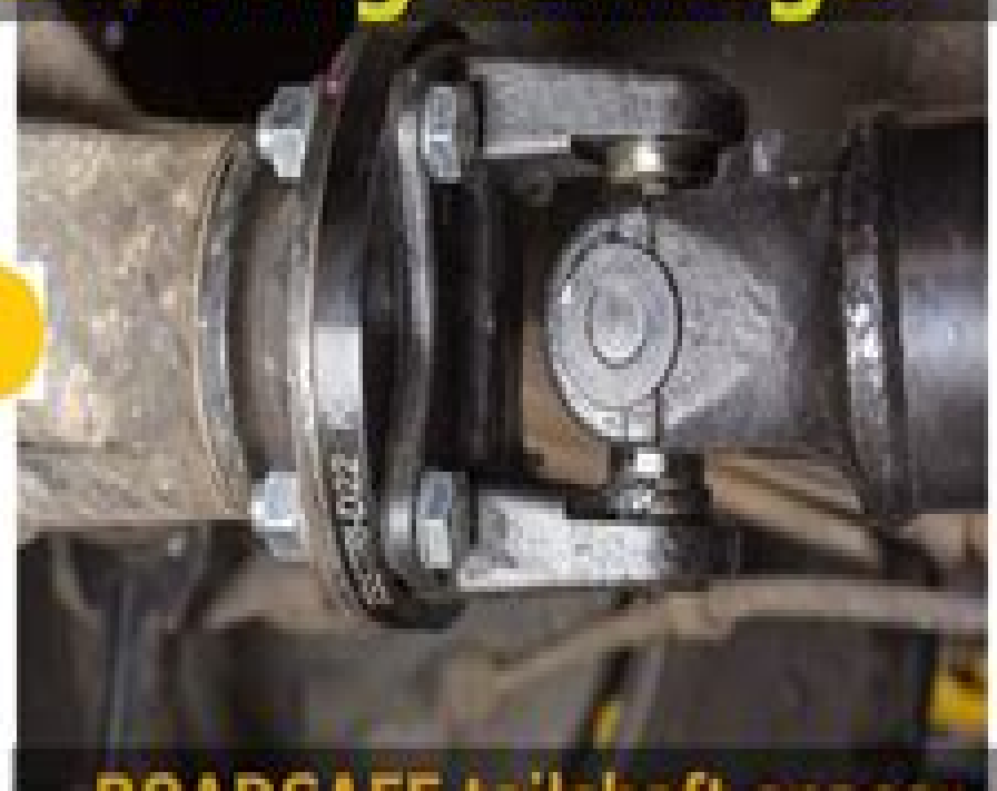
ROADSAFE tailshaft spacer TSSTRI installed
