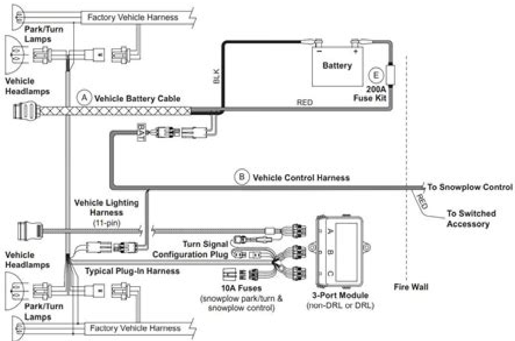
Vehicle-Side Harness Diagram
