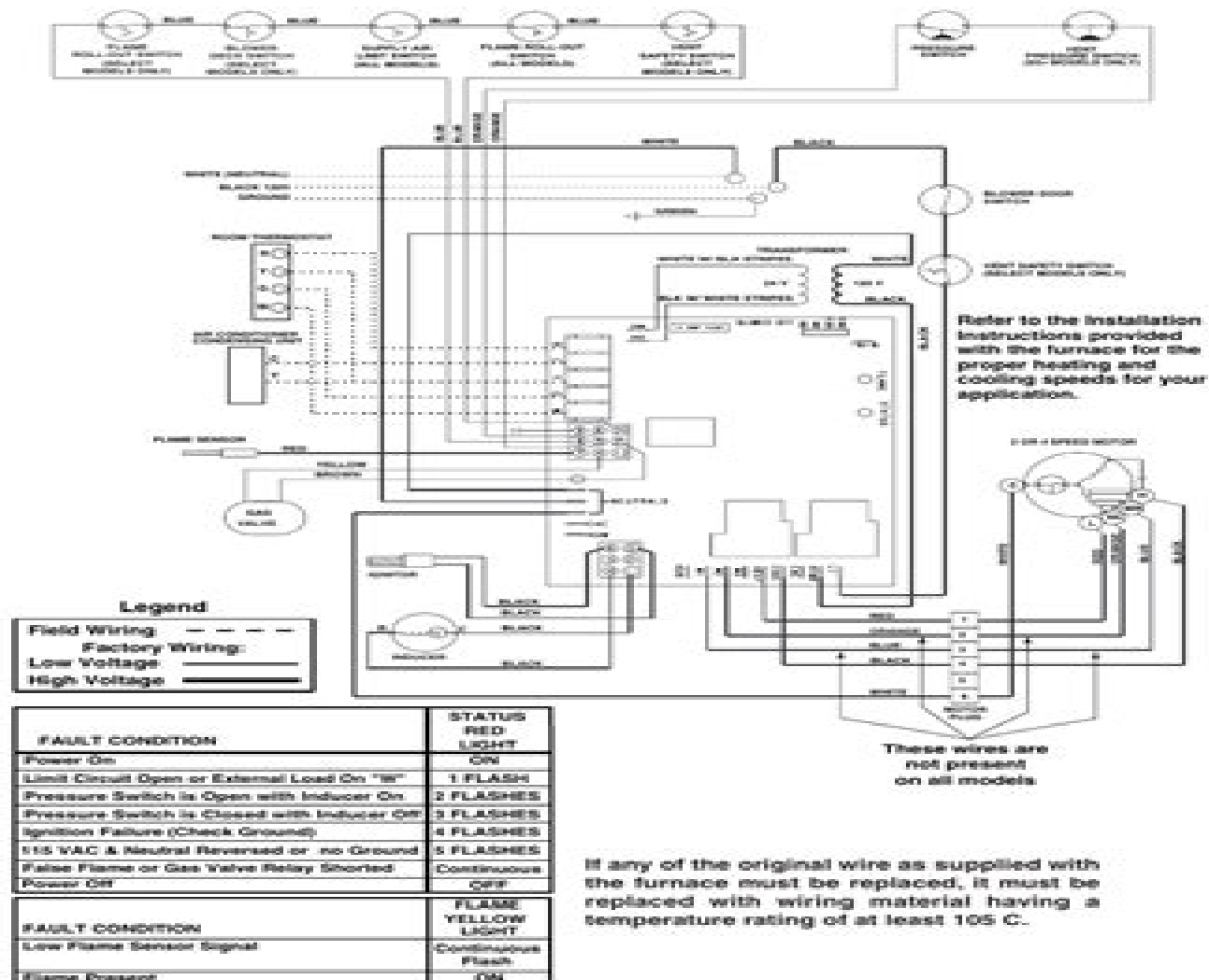
Figure 29. Upflow and Downflow Wiring Diagram
