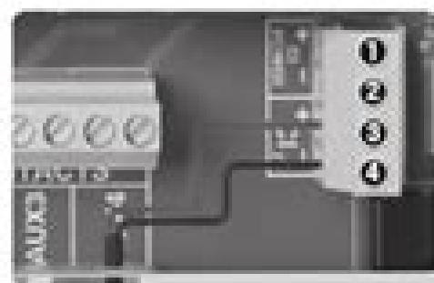
Free Chlorine probe ③ red ④ black
