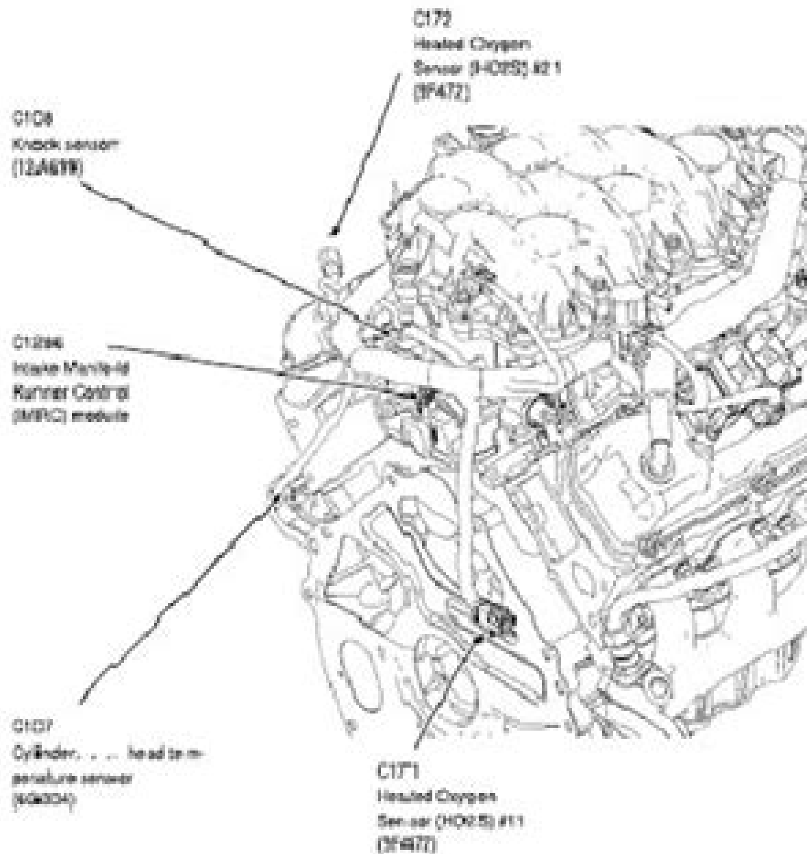
4.2L engine, rear
