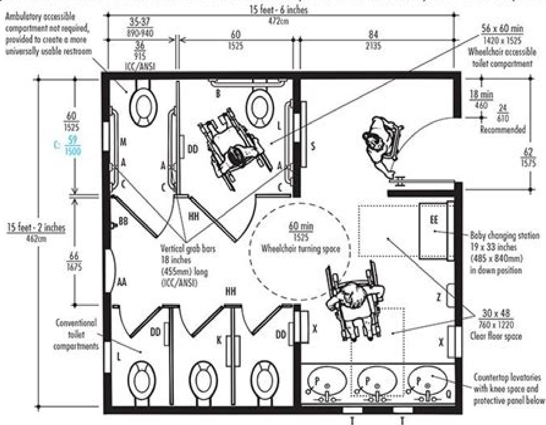
Fig. 19 Small Public Restroom Provides Accessible Toilet Compartment and Ambulatory Accessible Compartment.
