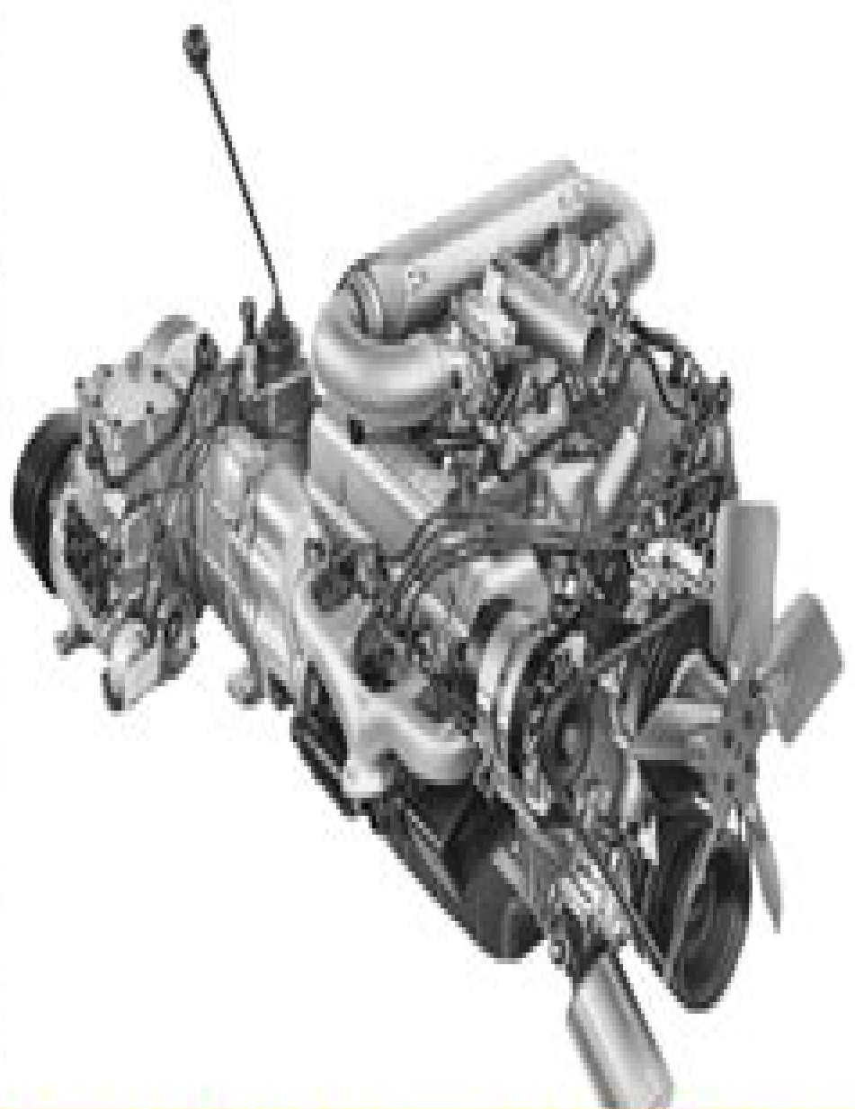
Rover V8 engine (Buick 215 V8) in the Range Rover Classic
