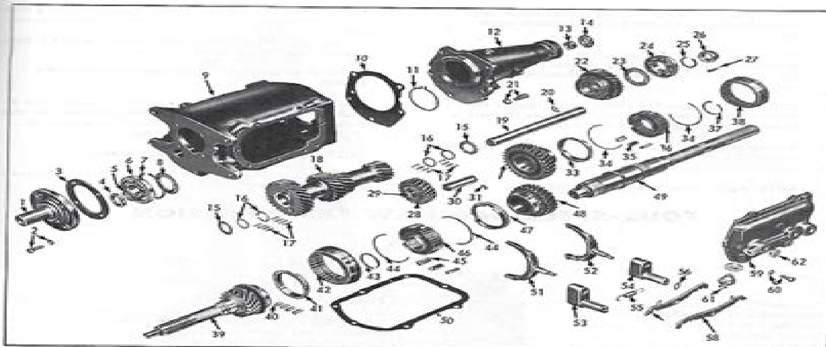
Fig. 6G—Transmission Exploded View
