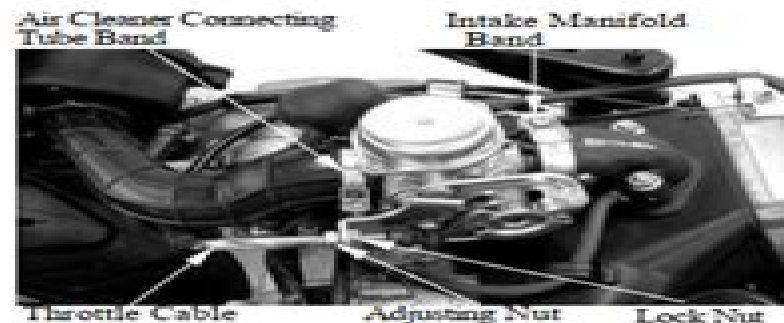
Throttle Cable
