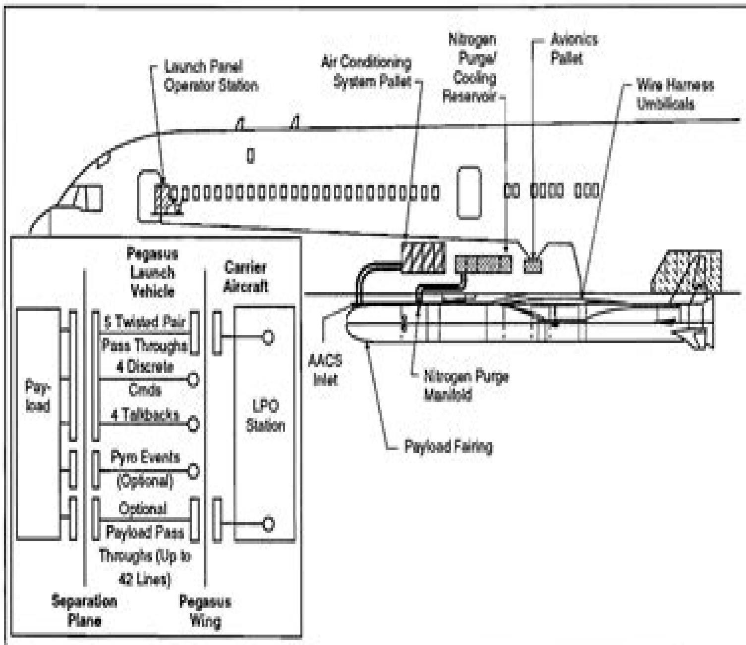
Figure 9. Pegasus/L-1011 Interface Details.
