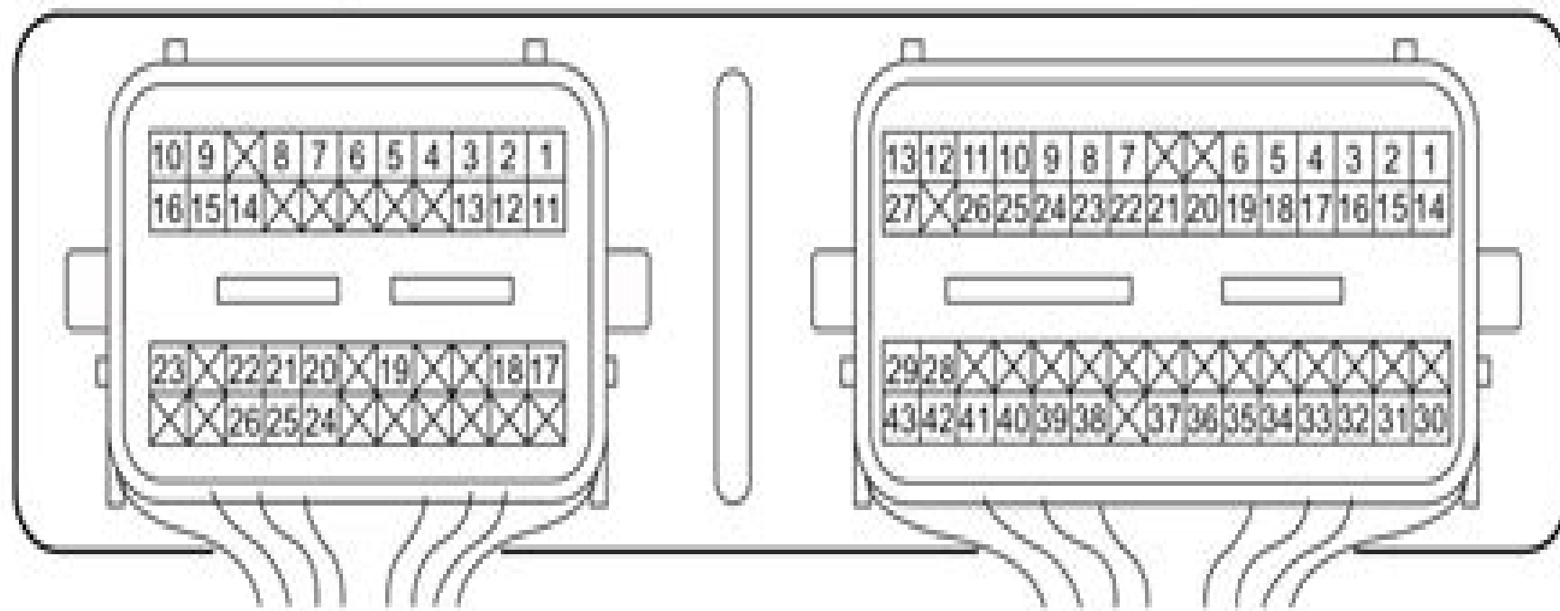
[A]: ECM connector (View: A)
