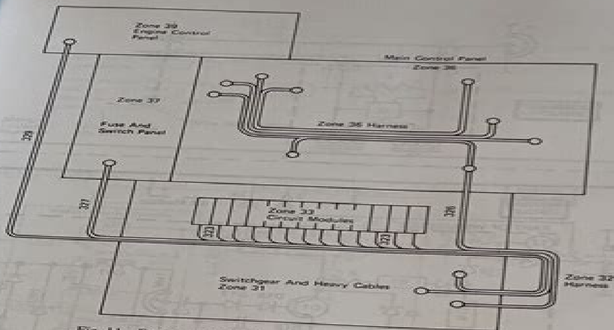
Fig. 11 - Equipment Location Zones, Electrical Cabinet (Units With Full Complement Of Plug-In Modules)
