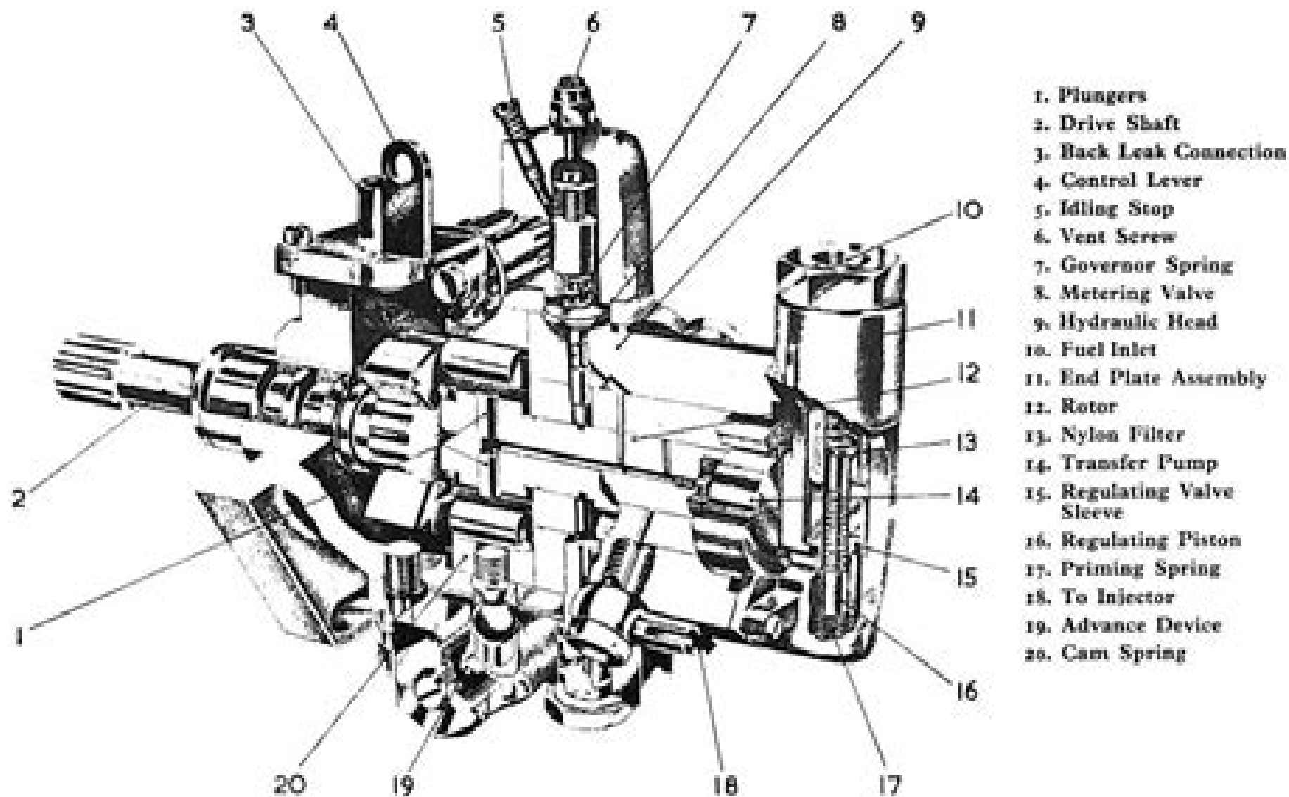
DPA pump with hydraulic governor and automatic advance device
