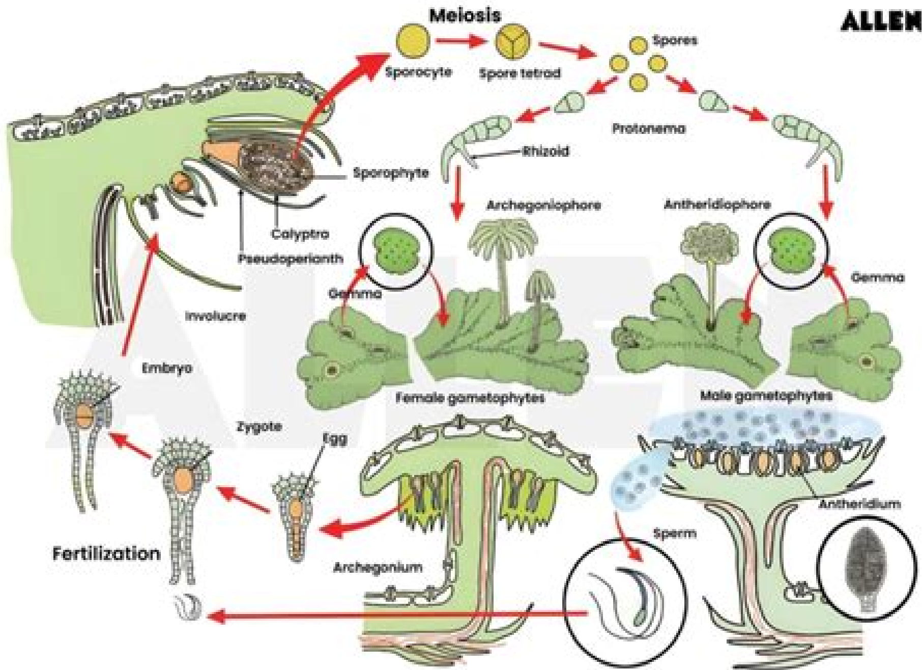
Figure :The Life cycle of Marchantia
