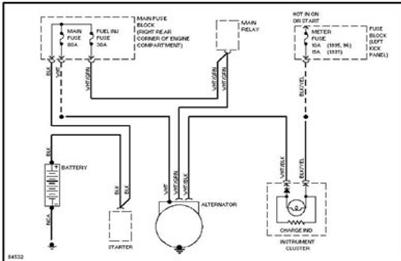
Charging Circuit
