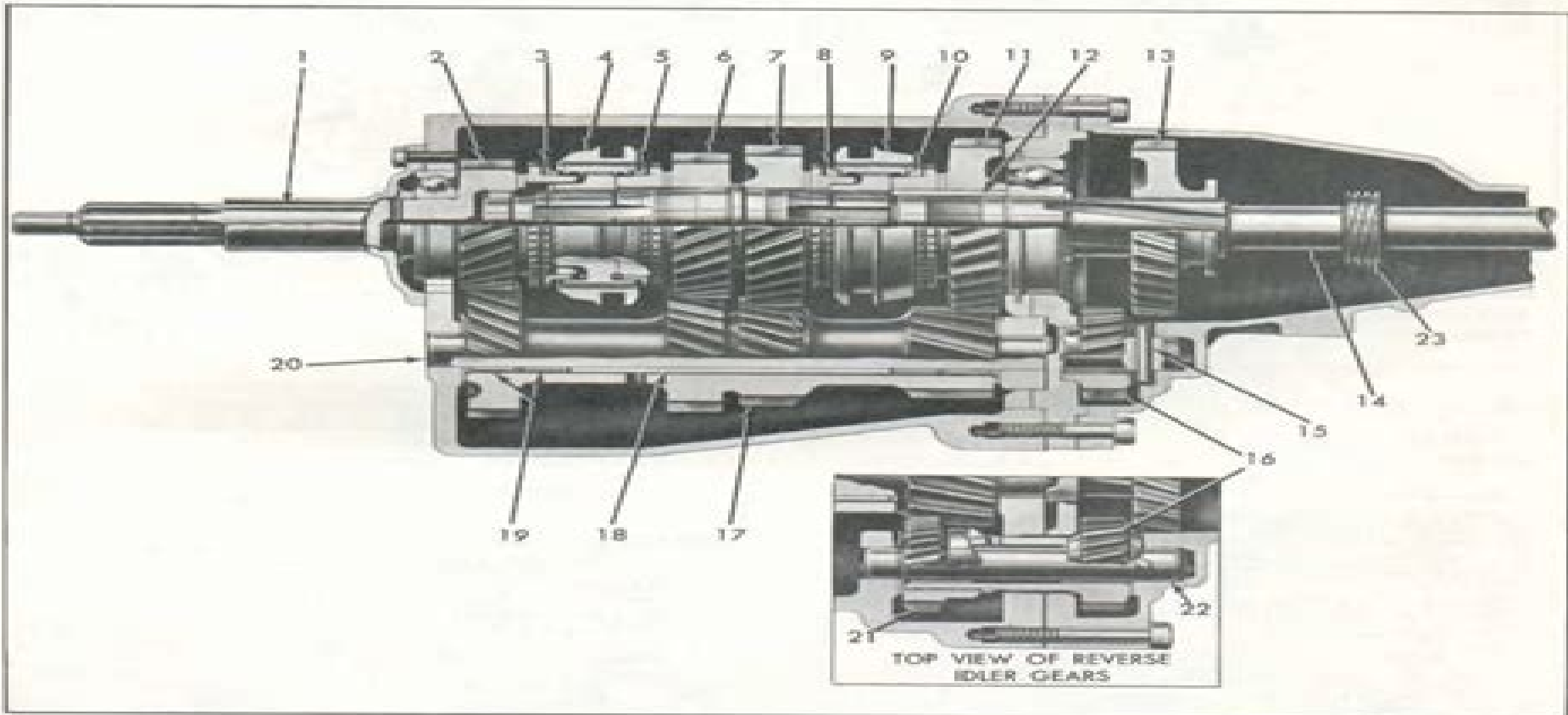
Fig. 1M—Four-Speed Transmission Cross Section (Close Ratio Shown)
