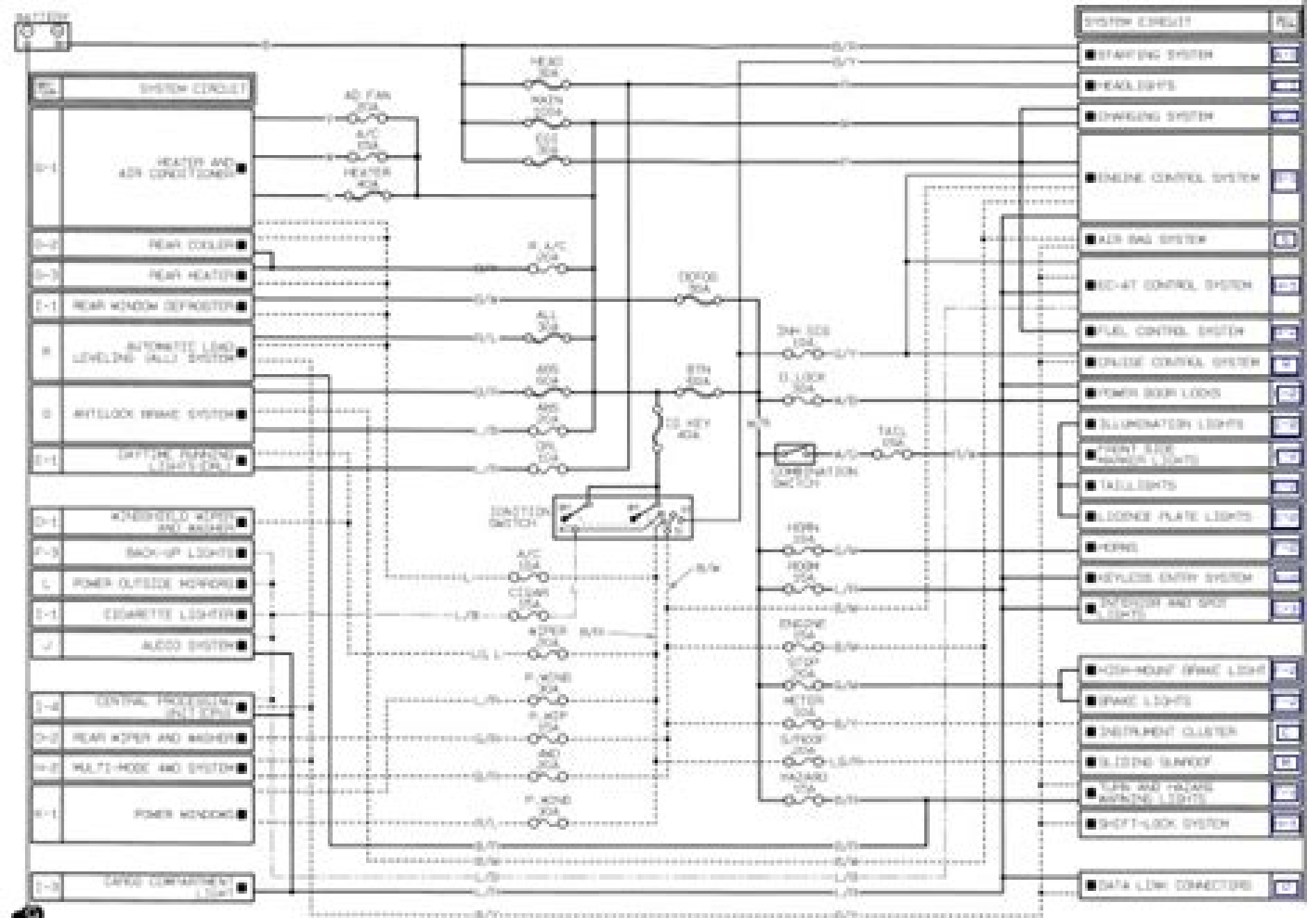
1996 MAZDA MPV WIRING DIAGRAM
