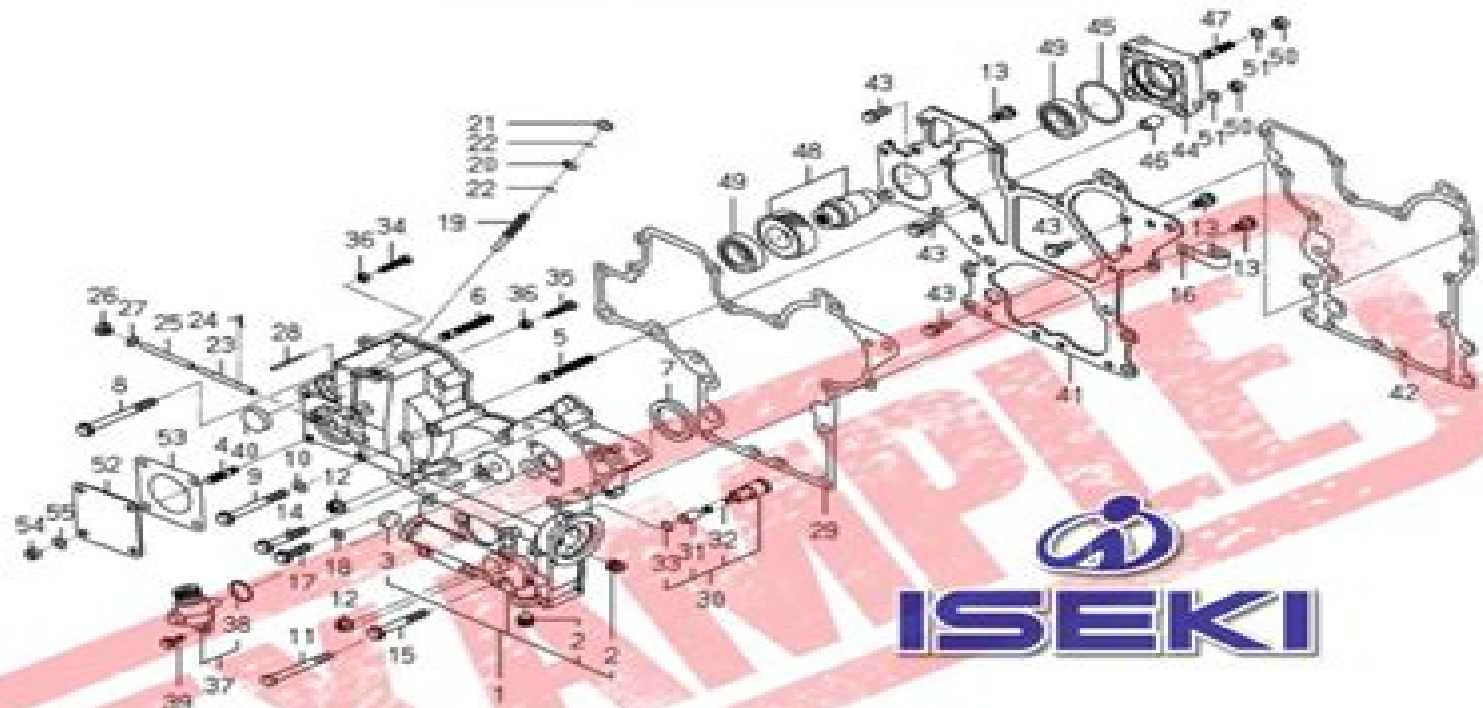
FIG. 9 TIMING GEAR CASE
