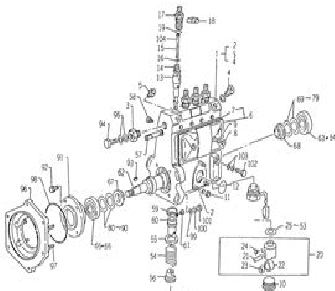
FIG. 16 COMPONENT PARTS FOR 6894 - 476 - 121 - 10 6897 - 030 - 187 - 00 ON Fig.14
