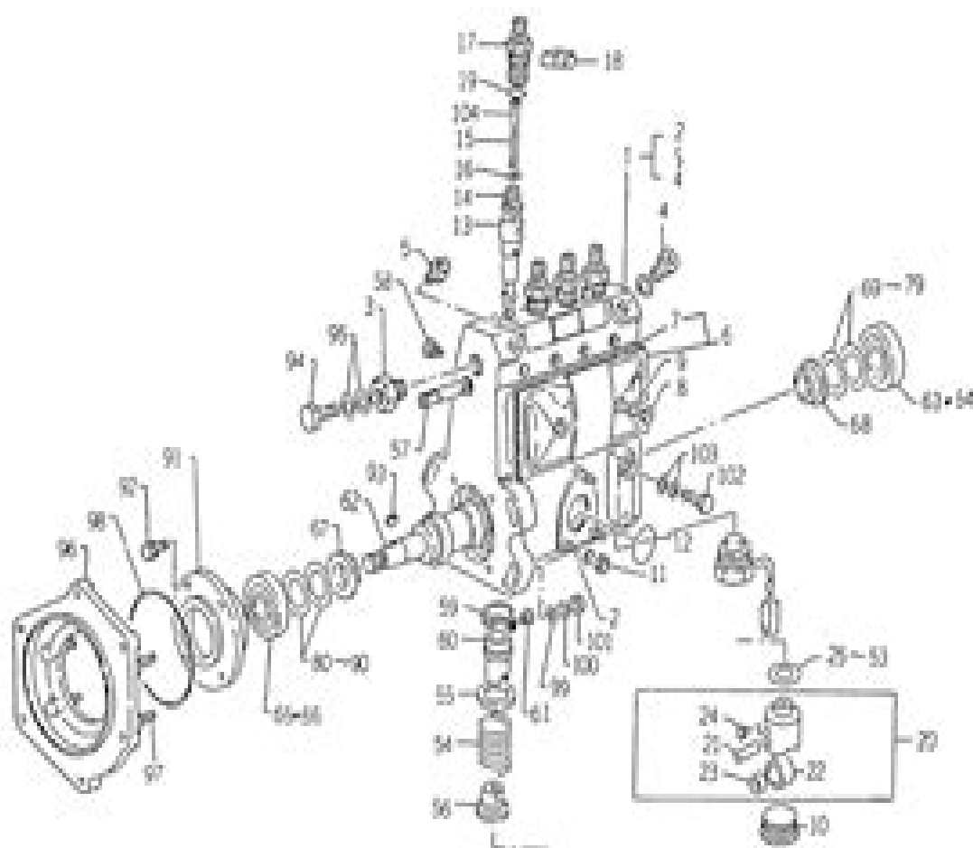
FIG. 16 COMPONENT PARTS FOR 6894-476-121-10 ON Fig.14 6897-030-187-00
