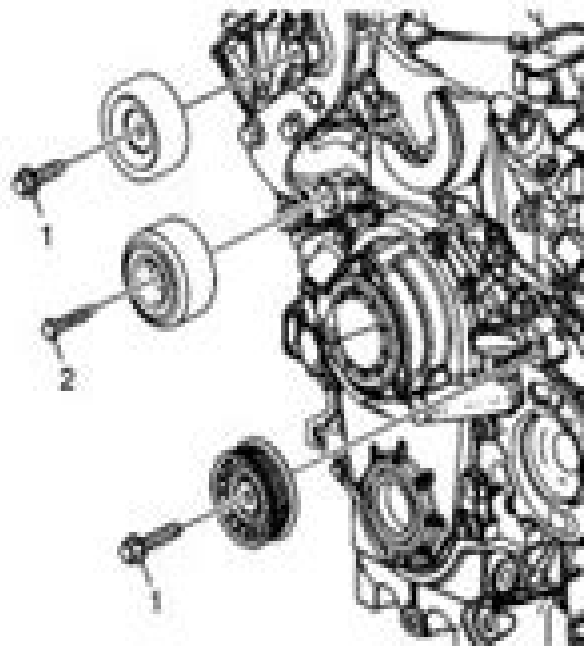
Fig. 427: Identifying Idler Pulley Bolts & Pulleys Courtesy of GENERAL MOTORS CORP.
