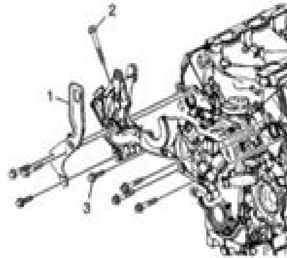
Fig. 428: Identifying Coolant Crossover Pipe Bolts Courtesy of GENERAL MOTORS CORP.
