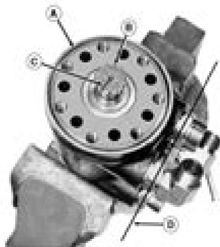
Steering Valve Timing
