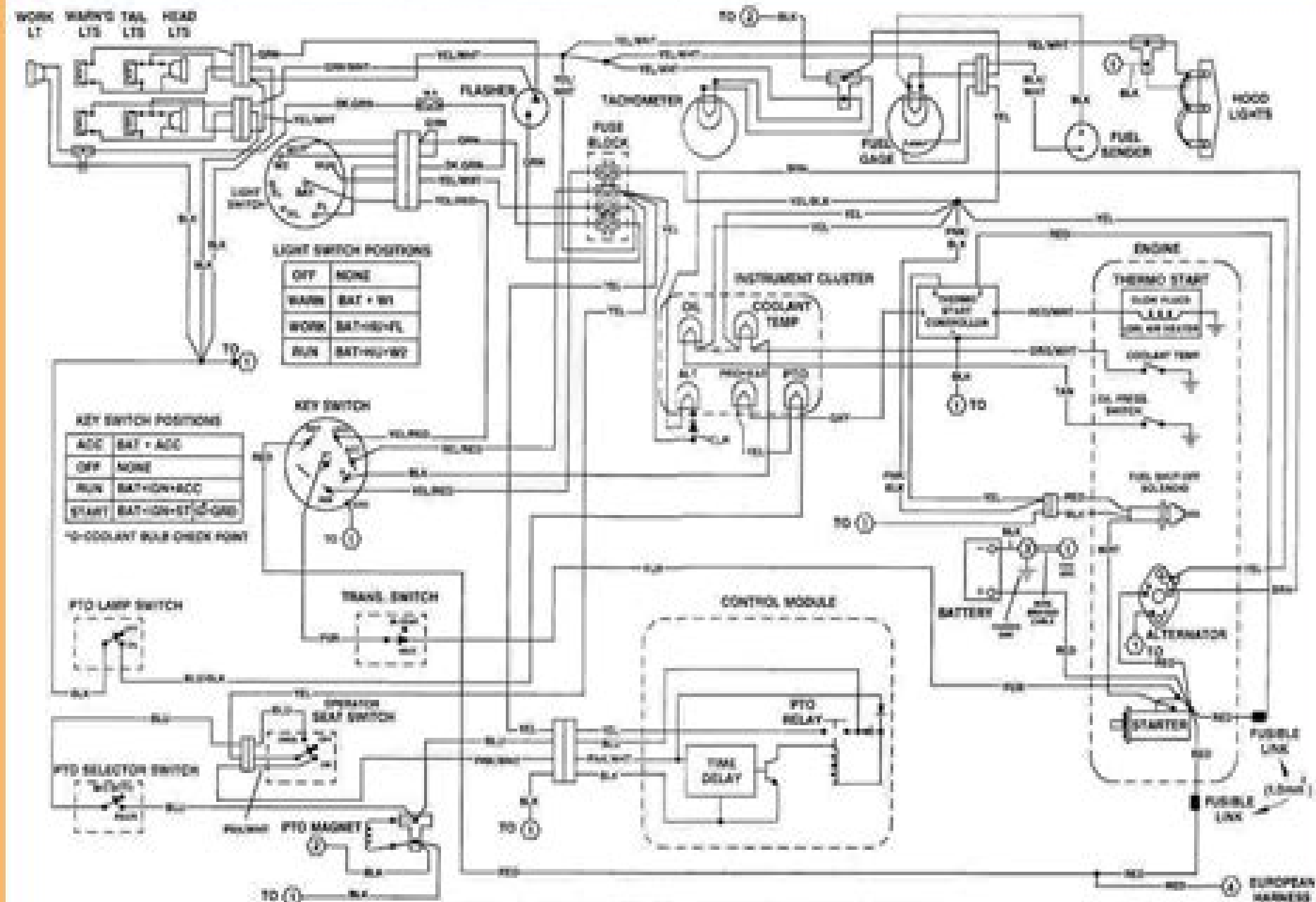
LATE 855 AND ORIGINAL 955 ELECTRICAL SCHEMATIC
