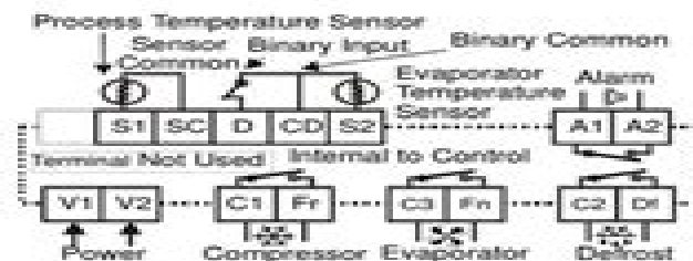
Figure 1: MR4 DIN Rail Mount Control
