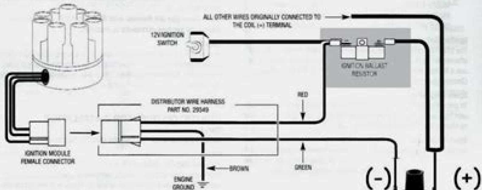
FIGURE 1 UNILITE® WIRING DIAGRAM USING BALLAST RESISTOR
