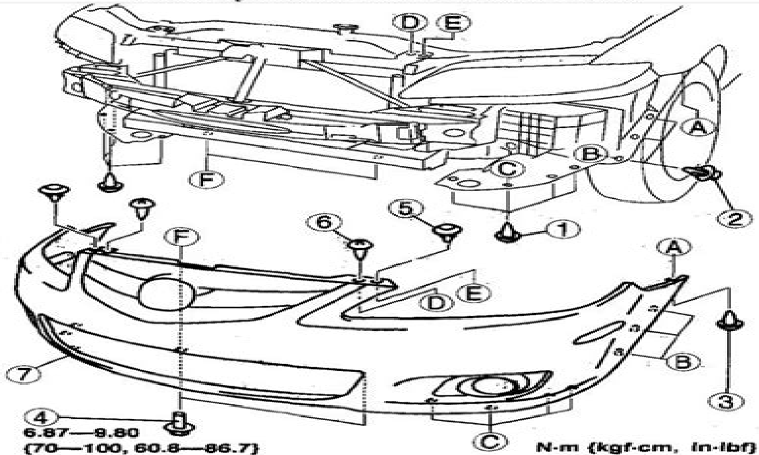
Fig. 22: Front Bumper
