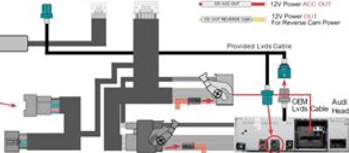
Audi Q5 Connector of Climate controller
