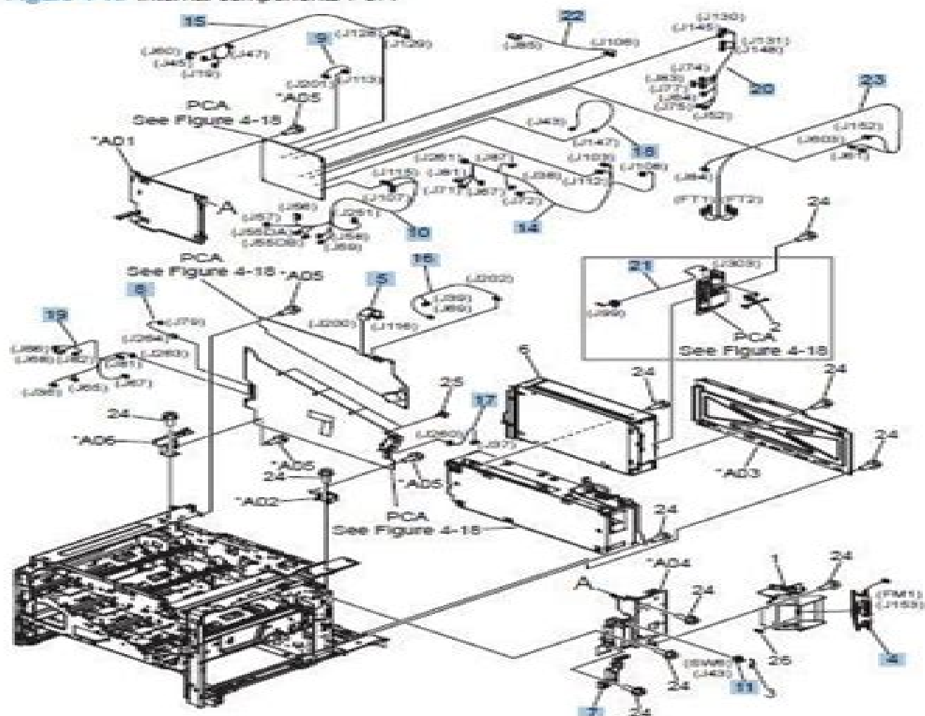
Figure 4-10 Internal components 7 of 7
