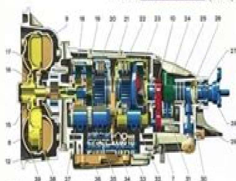
4-speed transmission with fluid coupling
