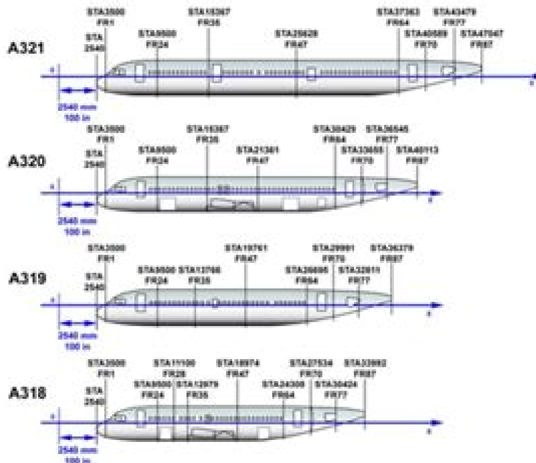
STRUCTURAL BREAKDOWN AND ZONING - FUSELAGE
