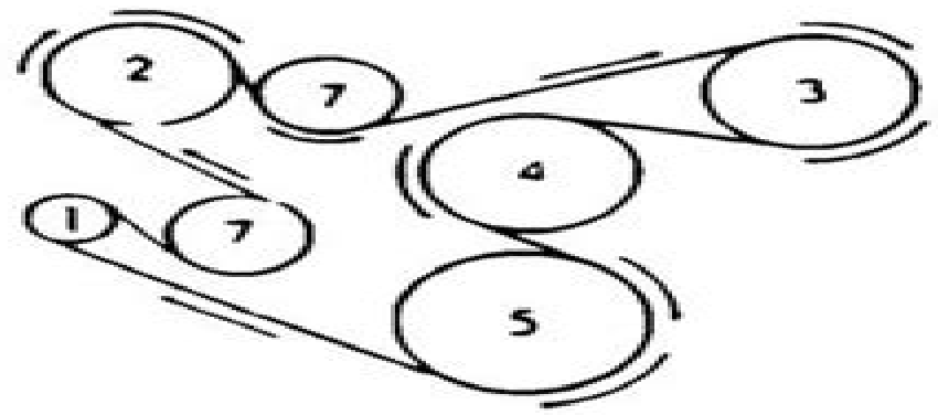
Grand Cherokee (With A/C)
