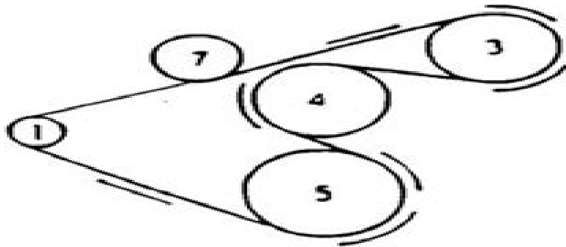
Cherokee & Wrangler (2.5L Engine) Grand Cherokee (Without A/C)
