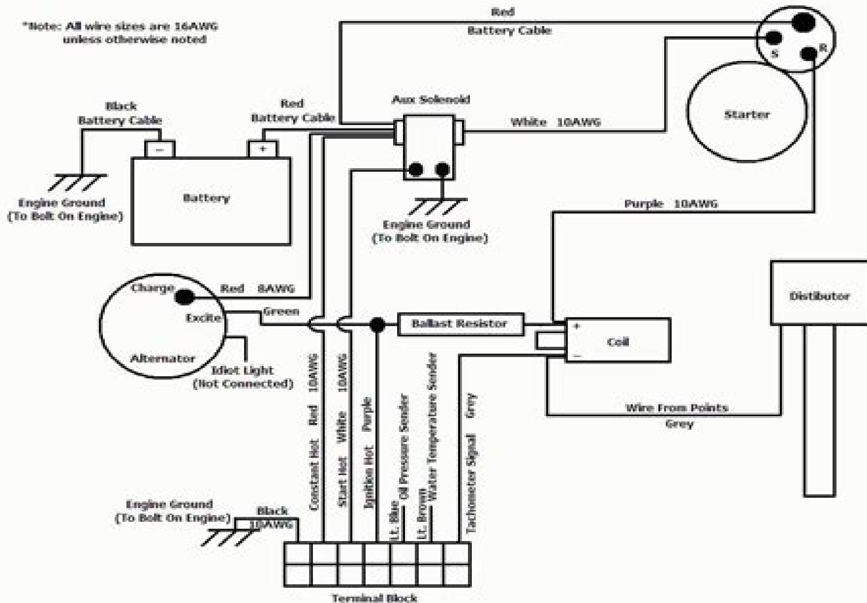
Typical Jet Boat Engine Harness 3-wire alternator, points ignition
