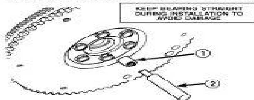
Fig. 6 PILOT BEARING INSTALLER
