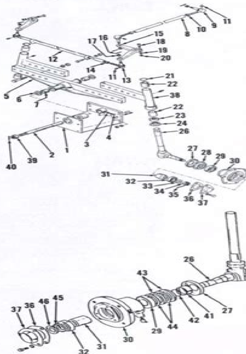
Fig. 3—Exploded view of spindle and hub components used on Model L210. For parts identification, refer to legend in Fig. 1 except for the following:
