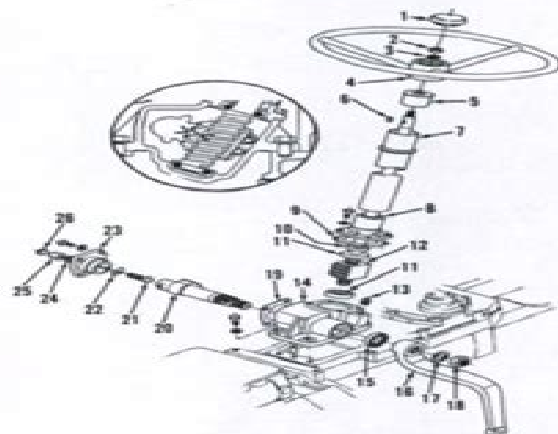
Fig. 4—Exploded view of recirculating ball nut steering gear used on Models L175, L225 and L225DT. Although details may differ, steering gear used on Models L210 and L260 is basically similar. During reassembly, align marks on sector shaft teeth (20) and worm gear (12) as shown in inset.
