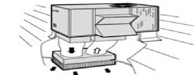
Down-Flow Supply and Return Air Installation with RMF16 Roof Mounting Frame, REMD16 Economizer and RTD11 Ceiling Diffuser.
