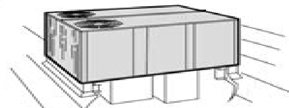
Down-Flow Supply and Return Air Installation with RMF16 Roof Mounting Frame.
