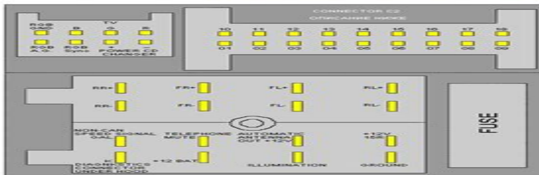
42 pin (8+8+18+8) Mercedes Comand ISO 7 proprietary connector
