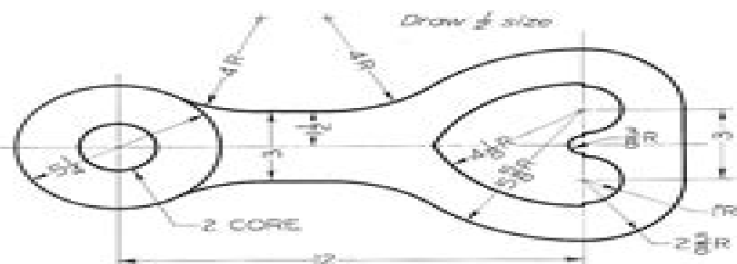
Fig. 5-37. Locomotive Truck Swing Link.*
