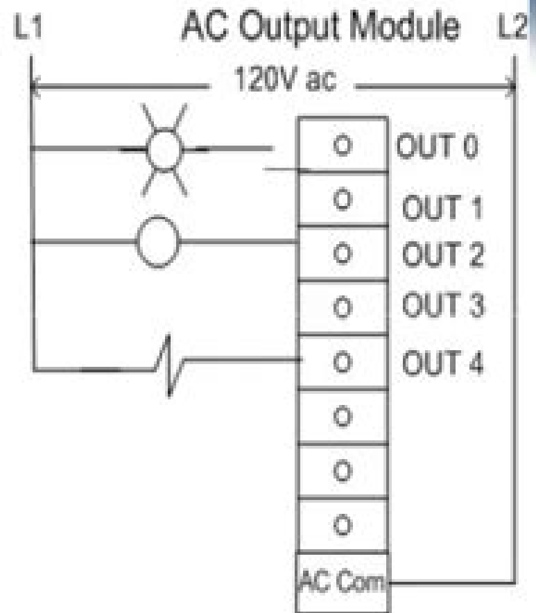
Figure 3.9 AC OUTPUT WIRING CONNECTIONS
