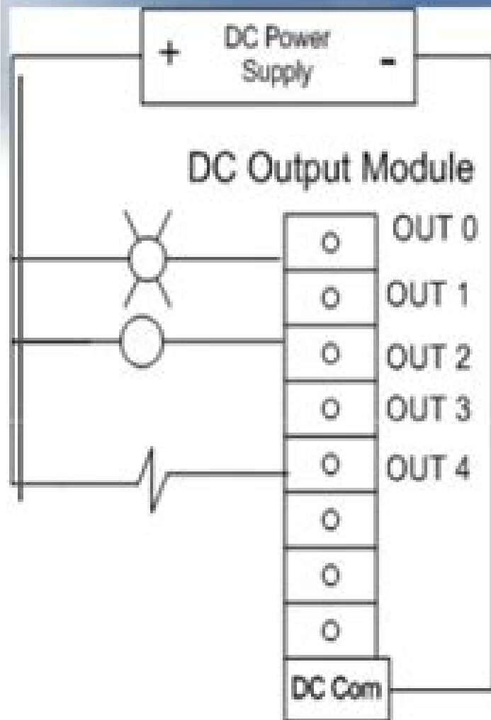
Figure 3.8 DC OUTPUT WIRING CONNECTIONS
