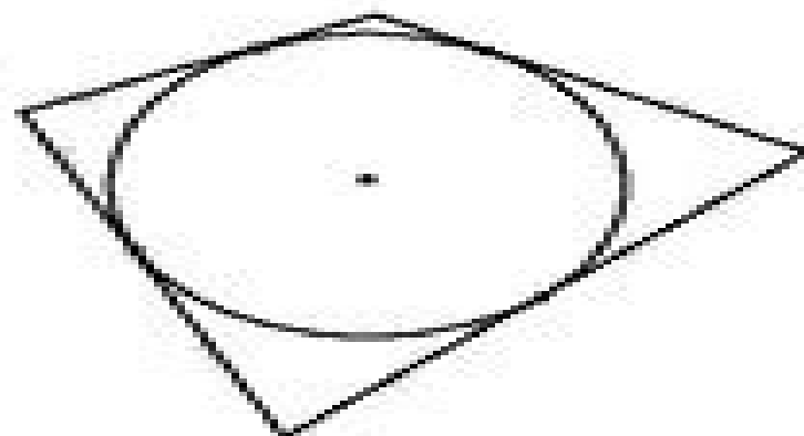
Circumscribed polygons
