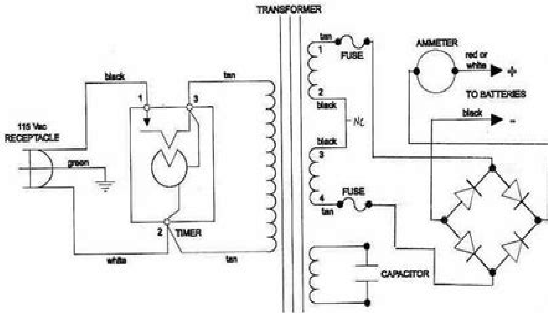
LESTER CHARGER 72 VOLT CHARGER (36LCT2512 MODIFIED)
